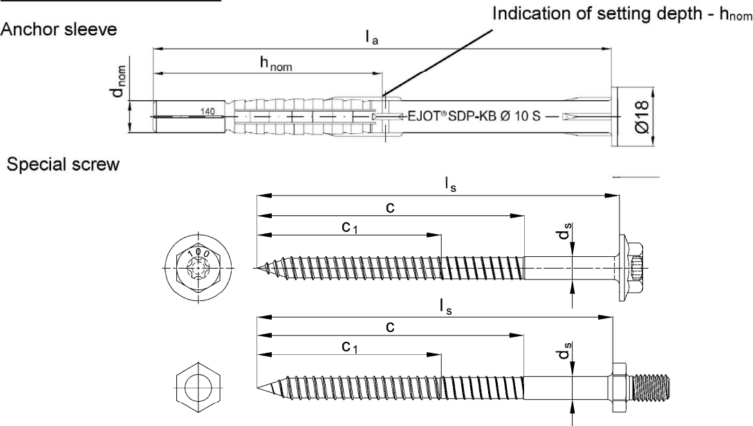
Picture 4: Dowel type collar head (KB)
